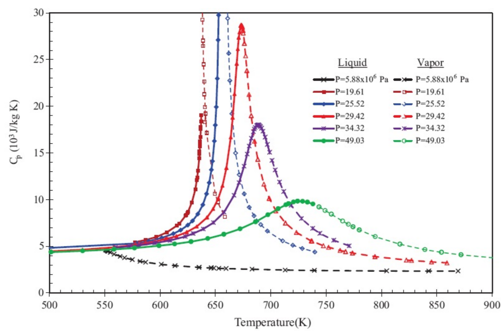
Figure 3. Experimental data for the heat capacity at constant pressure ( C_p ) of water (IAPWS, 2010). For a given pressure ( P ), the values are divided in two groups (a) for the compressed liquid region, shown by solid symbols and solid lines; and (b) for the superheated steam region, shown by empty symbols and dashed lines.
